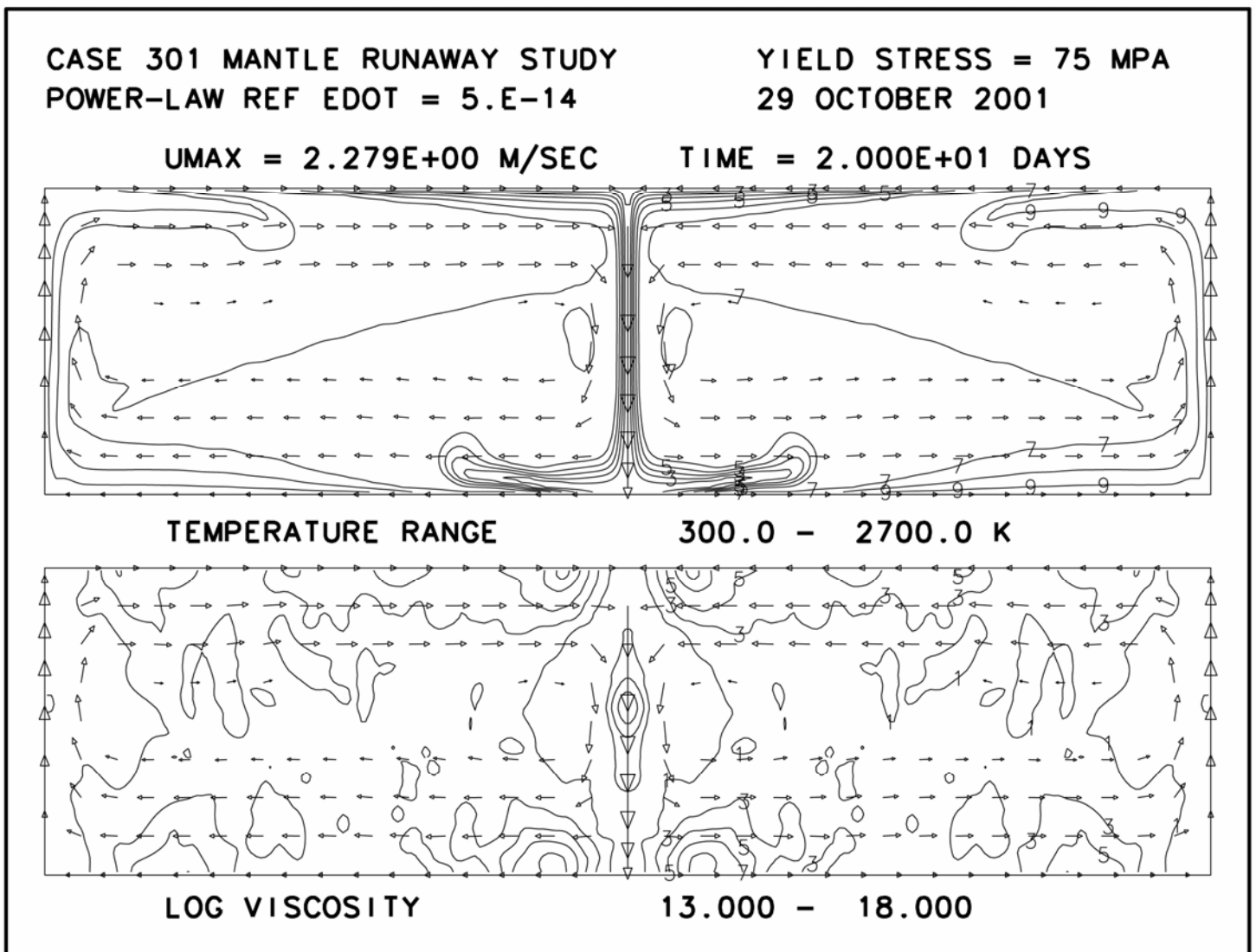
Figure 2. Three snapshots from a 2D mantle runaway calculation in a box 11560 km wide by 2890 km high at times of 5.0, 12.5, and 20 days. Arrows denote flow velocity scaled to the peak velocity 'umax'. Contours represent temperature in the top panels and base 10 logarithm of viscosity in the bottom panel. The viscosity range in the bottom panel plots is therefore 10^{13} to 10^{18} Pa-s.
