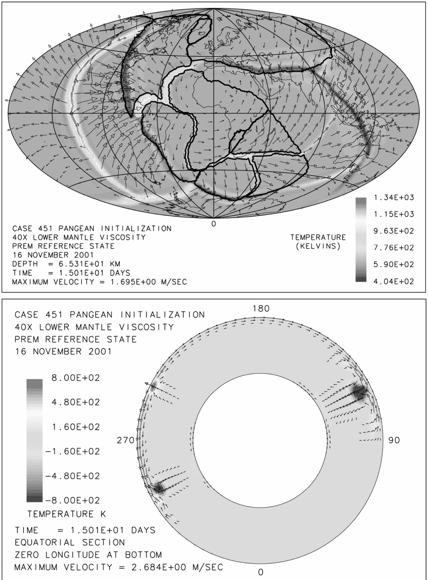
Figure 3(a). Snapshot of 3D solution after 15 days. The upper plot is an equal area projection of a spherical surface 65 km below the top surface in which grayscale denotes absolute temperature. Arrows denote velocities in the plane of the cross section. Arrows denote velocities. The dark lines denote plate boundaries where continental crust is present or boundaries between continent and ocean where both
