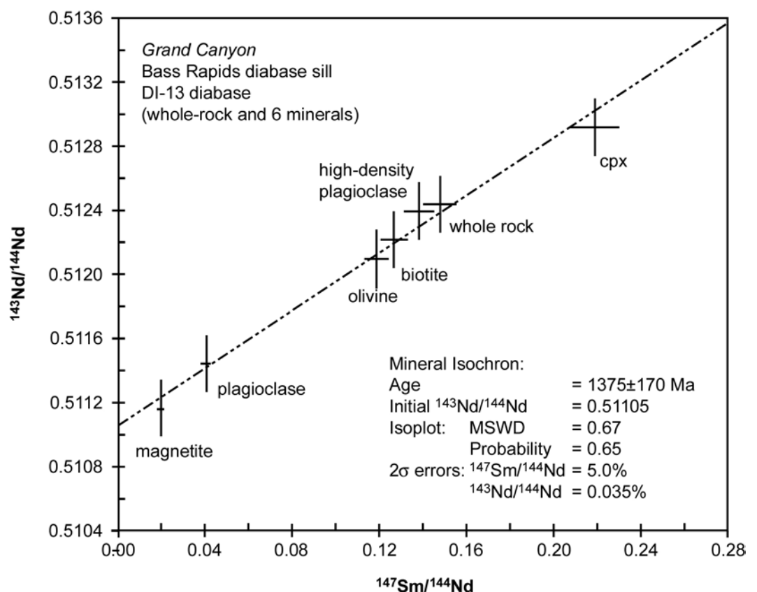
Figure 9. ^{147}\text{Sm}/^{144}\text{Nd} versus ^{143}\text{Nd}/^{144}\text{Nd} diagram for six mineral fractions from diabase sample DI-13 (plus the whole-rock) from the Bass Rapids diabase sill. All seven data points were used in the isochron and age calculations, and the bars represent the two-sigma uncertainties.
