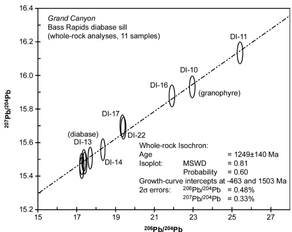
Figure 7. ^{206}\text{Pb}/^{204}\text{Pb} versus ^{207}\text{Pb}/^{204}\text{Pb} diagram for the Bass Rapids diabase sill, using all eleven whole-rock samples in the isochron and age calculations. The error ellipses represent the two-sigma uncertainties.
