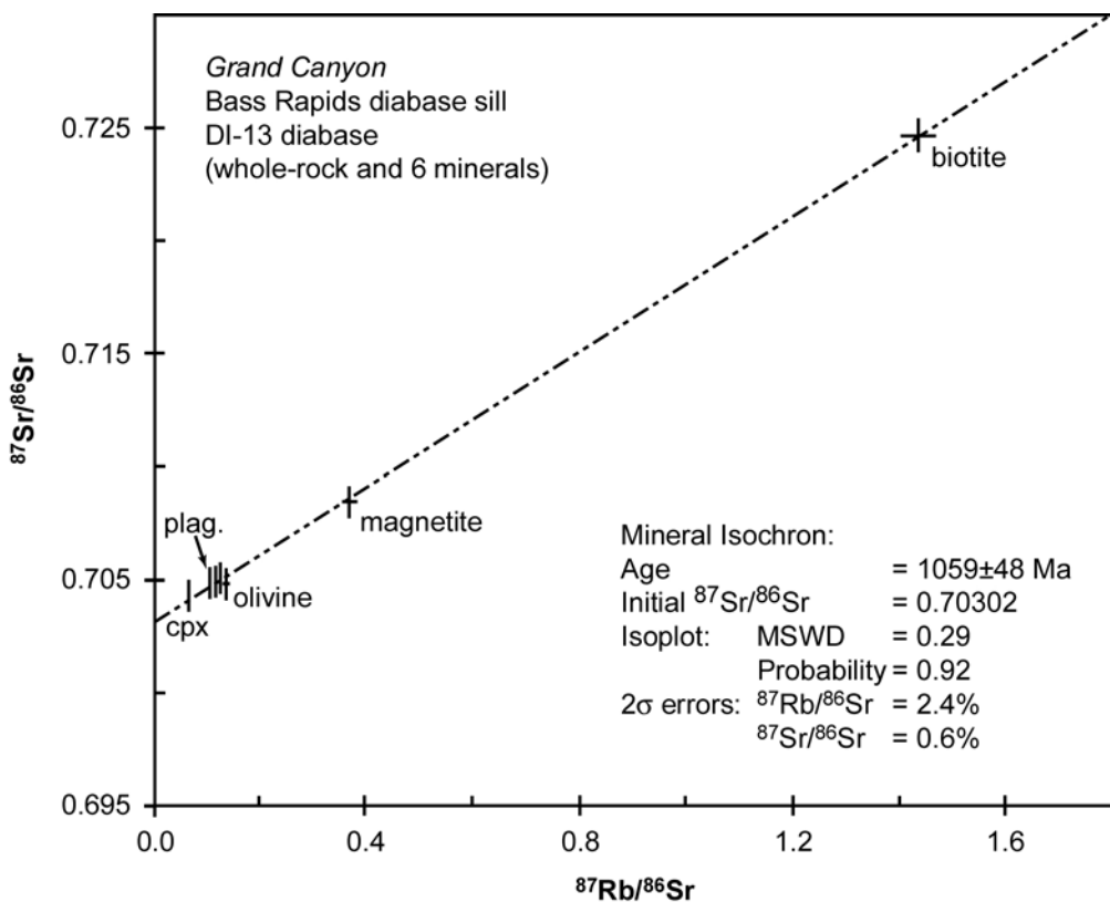
Figure 8. ^{87}\text{Rb}/^{86}\text{Sr} versus ^{87}\text{Sr}/^{86}\text{Sr} diagram for six mineral fractions from diabase sample DI-13 (plus the whole-rock) from the Bass Rapids diabase sill. All seven data points were used in the isochron and age calculations, and the bars represent the two-sigma uncertainties.
