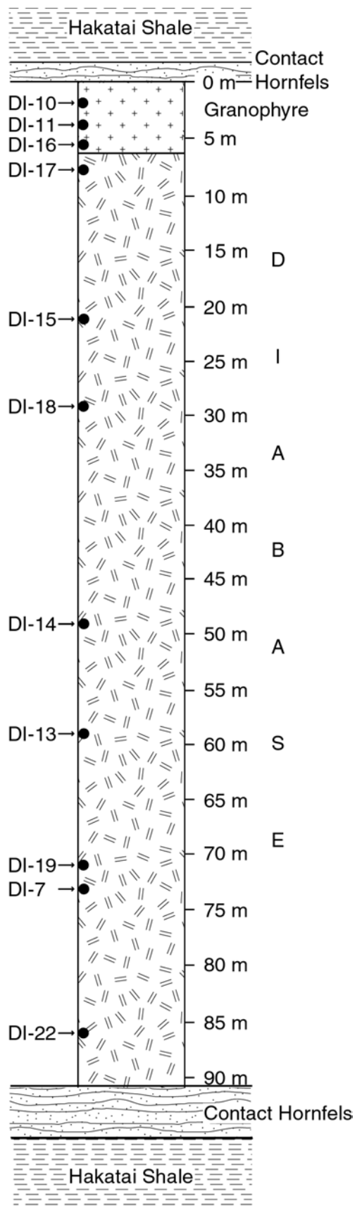
Figure 2. Diagrammatic section through the Bass Rapids sill showing the granophyre "capping" on the diabase, the contact hornfels, and the location of samples.
