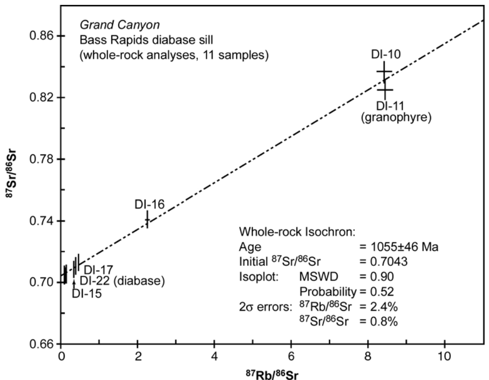
Figure 5. ^{87}\text{Sr}/^{86}\text{Sr} versus ^{87}\text{Rb}/^{86}\text{Sr} diagram for the Bass Rapids diabase sill, all eleven whole-rock samples being used in the isochron and age calculations. The bars represent the two-sigma uncertainties.
