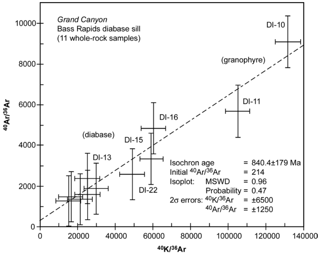
Figure 4. ^{40}\text{K}/^{36}\text{Ar} versus ^{40}\text{Ar}/^{36}\text{Ar} in the Bass Rapids sill, all eleven samples being used in the isochron and age calculations. The bars show the two-sigma uncertainties.
